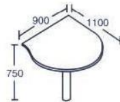
Connection Top with Metal Leg (Left & Right) CT1100 L1100 x W900 x H750
