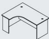
BE LT1512-R Ergonomic Table-Right W1500 L1200 D700/450 H750
